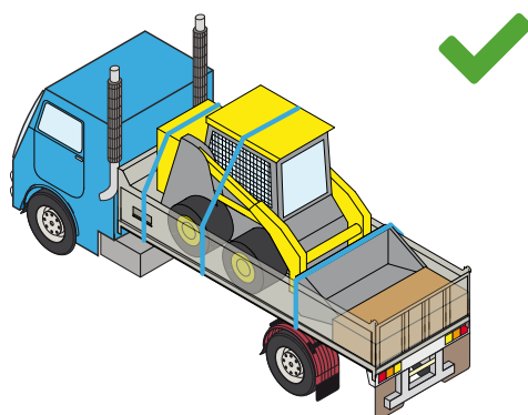
Figure 185 Suspended load
