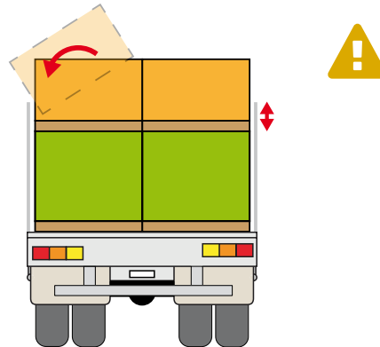
Figure 183 Lashed gates
