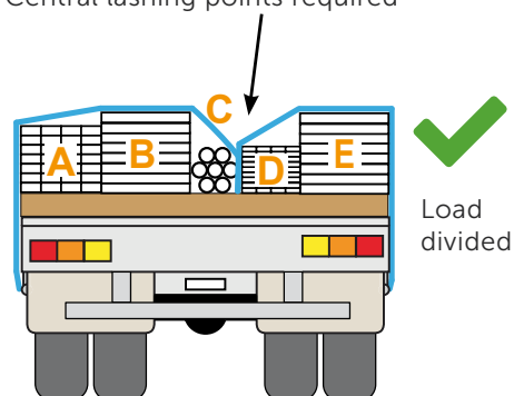
Figure 131 Divide loads
