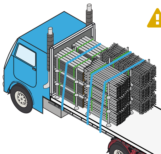
Figure 339 Stacked H-frames
