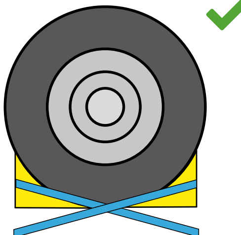
Figure 302 Chocks restrained
