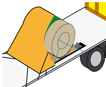
Figure 403 Cap tarpaulin
