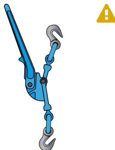
Figure 454 Over-centre lever binder (dog)
