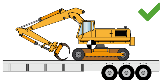
Figure 253 Excavator on low loader
