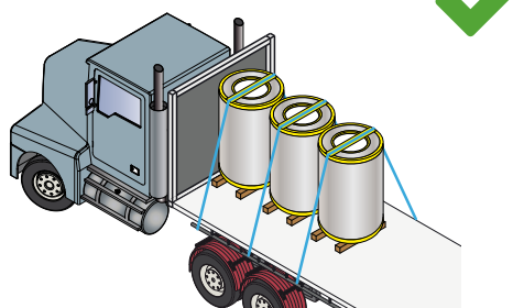
Figure 82 Blocked rolls tied down
