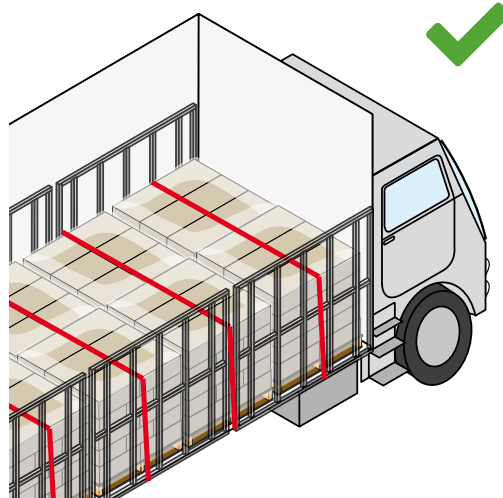
Figure 363 Tie Down lashing containing gates without affecting lashing angle
