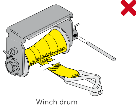
Figure 417 Webbing layered unevenly
