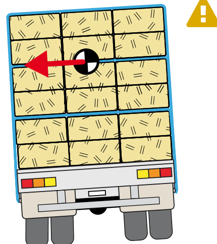
Figure 168 High-centre-of-gravity load
