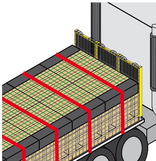
Figure 379 Headboards used with tie-downs can safely restrain heavier loads than when used without tie-downs
