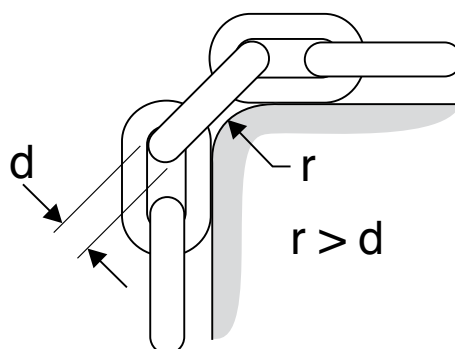
Figure 434 Derating of chain
