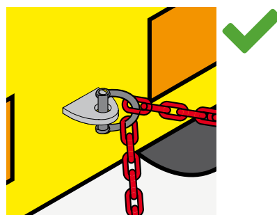
Figure 264 Towing bracket shackle lashing point
